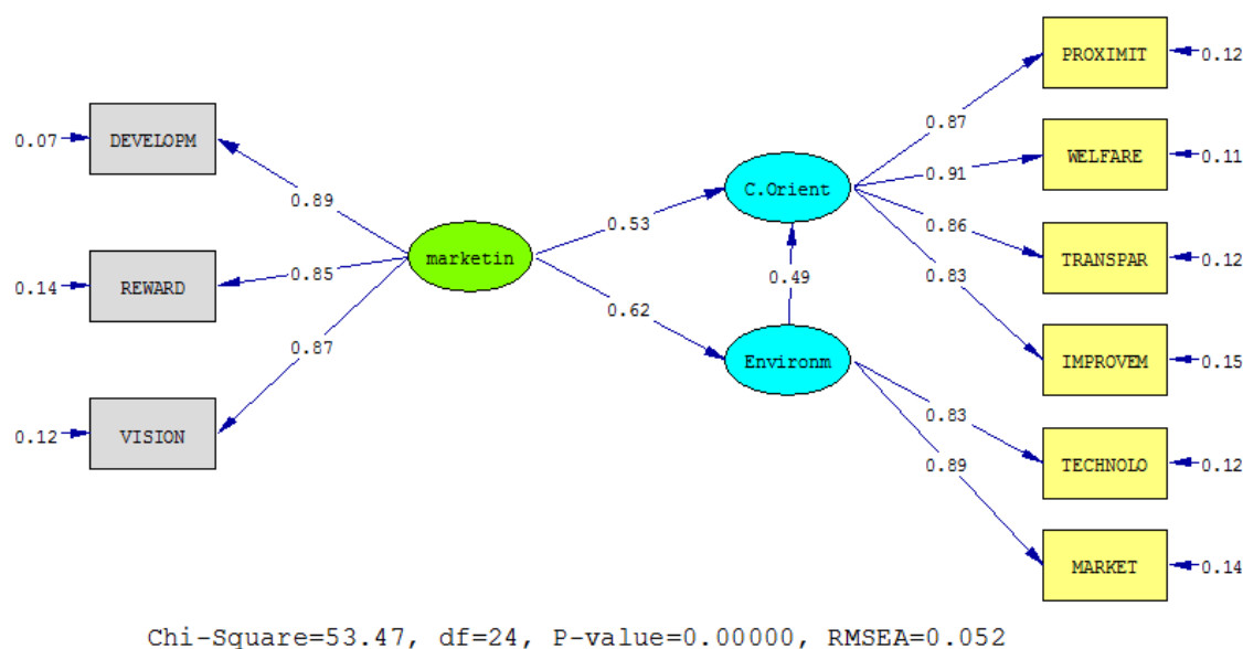
Figure 2: The Main Model in Standardized Form
